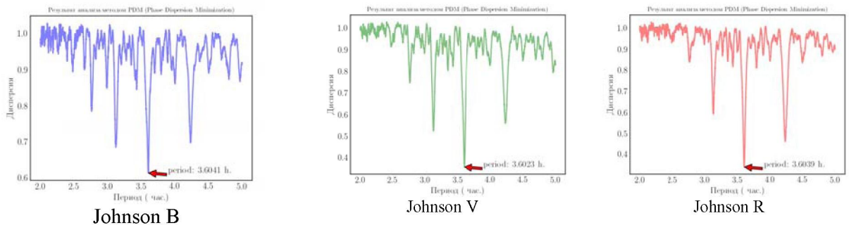
Figure 3 - The results of determination of the period of Phaethon's differential magnitude variations in filters B, V and R (designations under the corresponding panels) shown in Figure 2, by the PDM (Phase Dispersion Minimization) method.
