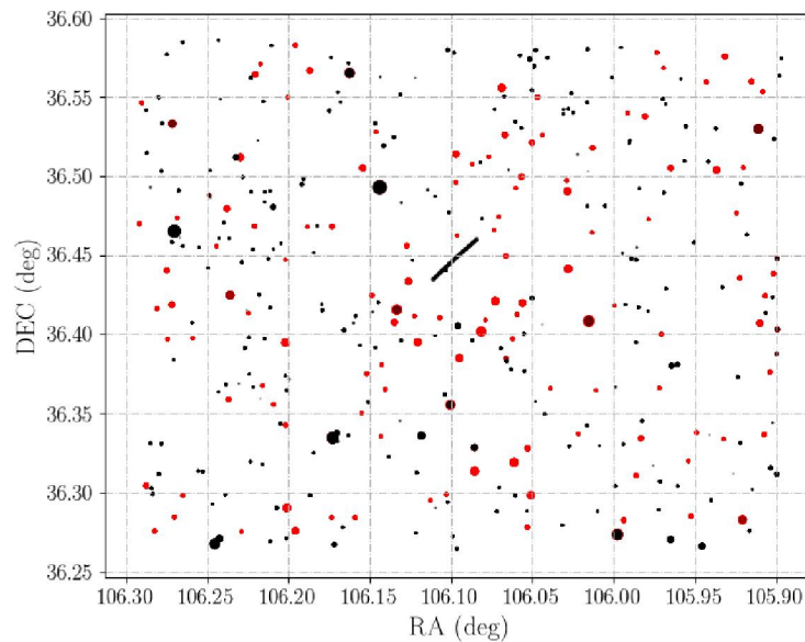
Figure 1 - Map of sources that have passed the procedure of photometry and astrometry. Catalog stars are indicated by colored symbols. Sources not included in the catalog are indicated by black symbols. The size of the symbols depends on the instrumental stellar magnitude. Asteroid track is visible in the center of the frame. The results of observation on 20.11.2017 TSO ("Eastern" Zeiss-1000).
