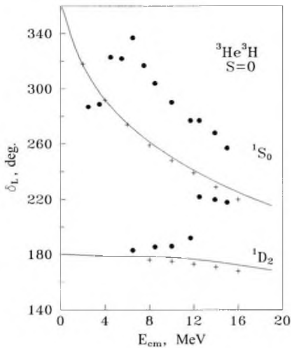
Figure 1c - Phase shifts of the {}^3\text{He}{}^3\text{H} scattering. Curves are calculations for potentials with parameters from table 1. Points are experimental data from [17,18]. Crosses are RGM calculations from [19]
