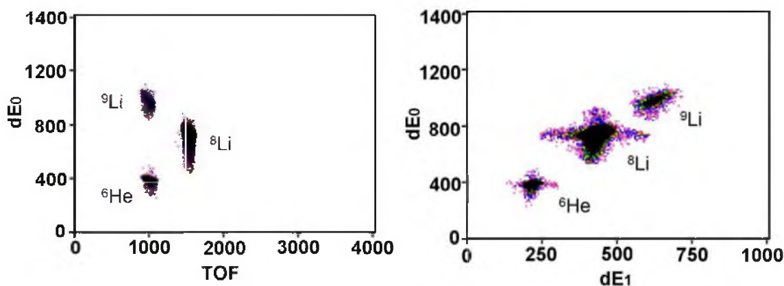
Figure 2 – Two-dimensional spectra of identification detectors dE_0 and dE_1 : energy losses in dE_0 and TOF (left) and energy losses in the detectors ( dE_0 \times dE_1 ) (right). The spectra demonstrate good separation of {}^6\text{He} and {}^{8,9}\text{Li} nuclei formed as products of ( {}^{11}\text{B} + {}^9\text{Be} ) reaction
