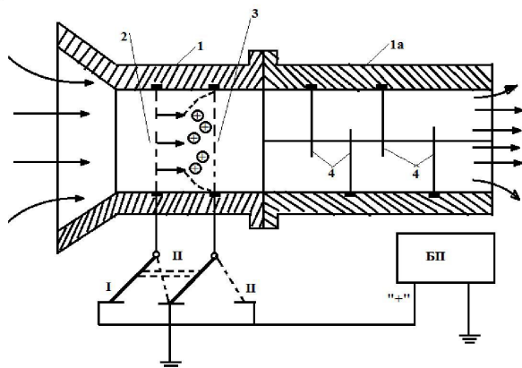
Figure 1 – Functional scheme of the device
