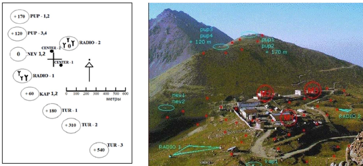
Figure 12 – Disposition of detectors layout on TShHSS for the thunderstorm phenomena registration
