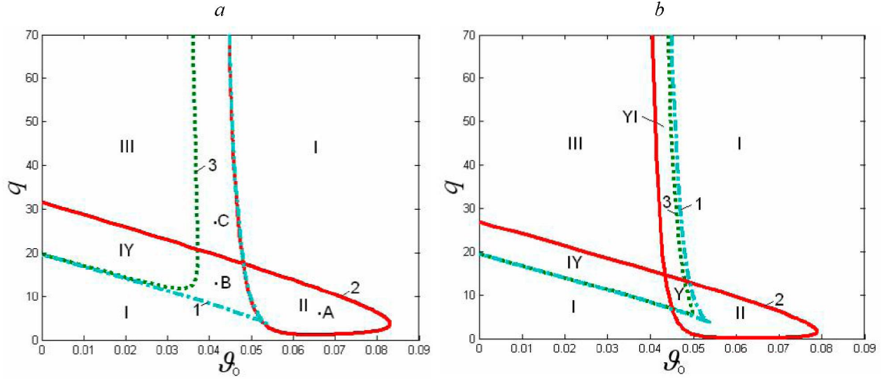
Fig. 2. Stability regions for different values inlet coolant flow velocity.
