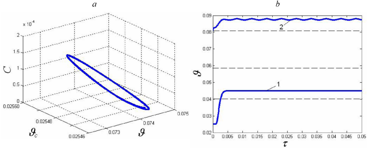
Fig. 4. Phase portrait of auto-oscillating regime, corresponding point A (a) and multiple regimes, corresponding point B in Fig. 2,a (b). a) q = 7 ; g_0 = 0,067 ; x = 0,6 ; b) q = 14 ; g_0 = 0,042
