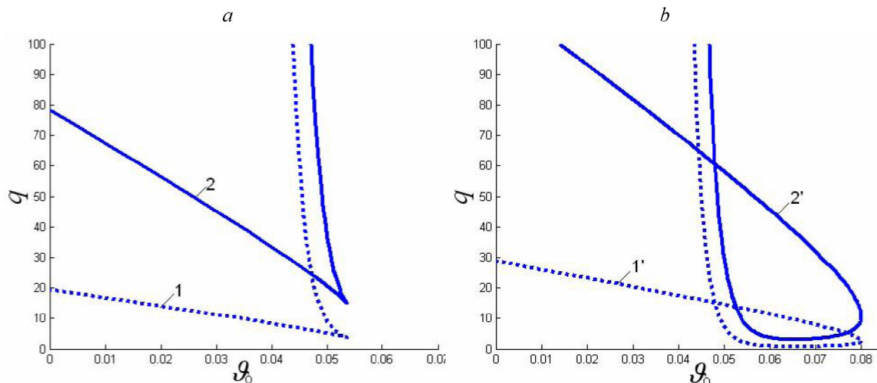
Fig. 3. Influence of inlet reactant mixture concentration C_0 on non-unique (a) and neutral stability (b) boundaries: C_0 = 0.004 (1,1'); 0.001 (2,2'); other parameters corresponding Fig. 2, a
