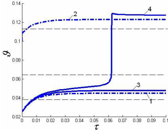
Fig. 5. Sensitivity of reactor to change of coolant temperature: 1, 2 – high- and low temperature stable regimes corresponding point C in Fig.2,a: x=0,6 ; g_{c0} = 0,025 (1,2); 0,04 (3); 0,055 (4)
