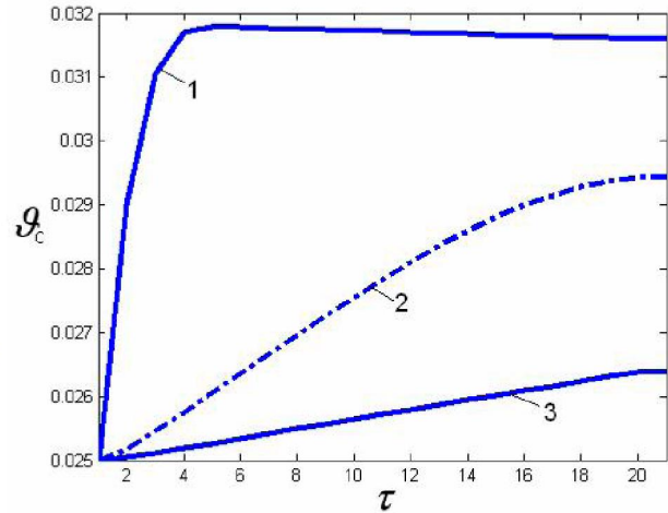
Fig. 6. Influence of inlet coolant flow velocity on coolant temperature: x=0,6 ; Pe_c=0 (1); 30 (2); 130(3). Other parameters corresponding point C in Fig. 2, a
